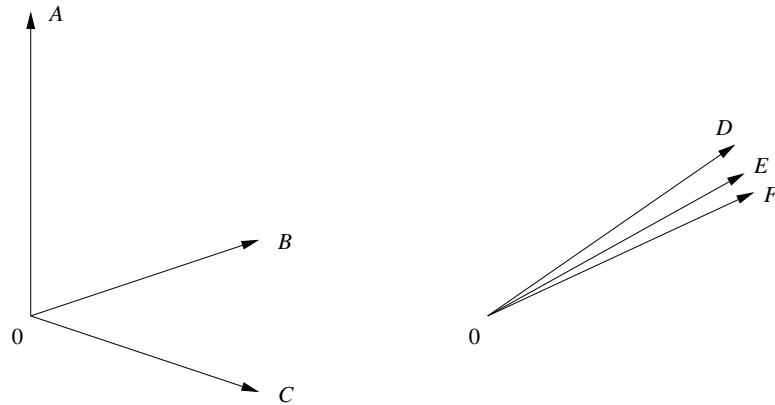
Figure 1.2. Orthogonal vectors in 3-space compared with 3 similar vectors.
